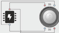
Parallel wiring → 1 Ohm
