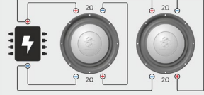
Parallel / serial mixed wiring → 2 Ohms
